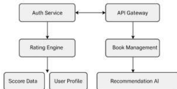
Figure 1. Microservices-based Architecture of the Platform
